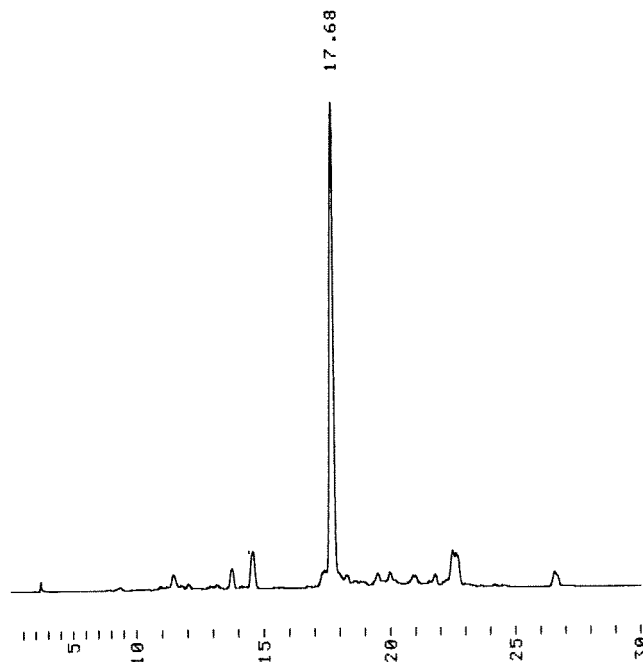
Figure 2. HPLC chromatogram of the crude synthesis product of conjugate 33 (refers to a pair of stereoisomers). Hypersil Hypurity C18 (150 \times 4.6 mm, 5 \mu\text{m} ), gradient from aqueous 0.1% TFA to acetonitrile in 30 min, flow 1.0 mL \text{min}^{-1} , detection at 276 nm.
