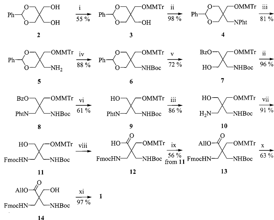
Scheme 1. Synthesis of building block 1 . (i) MMTTrCl, Py, (ii) PhthNH, DEAD, Ph 3 P, THF, (iii) NH 2 NH 2 , OH 2 , EtOH, (iv) Boc 2 O, NaOH, H 2 O, MeCN, (v) t BuOOH, Pd(OAc) 2 , benzene, (vi) NaOMe, MeOH, (vii) FmocCl, DIPEA, dioxane, (viii) PDC, DMF, (ix) AllBr, DIPEA, DMF, (x) I 2 , MeOH, (xi) CrO 3 , H 2 SO 4 , acetone.
