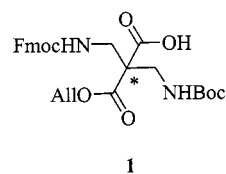
Figure 1. Orthogonally protected bis(aminomethyl)malonic acid ( 1 ).
