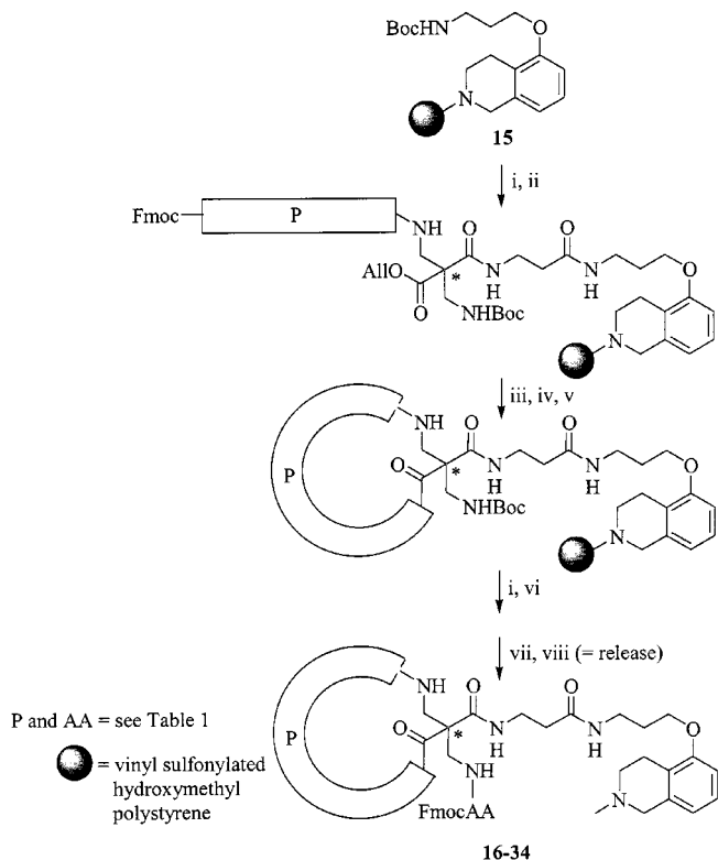
Scheme 2. Synthesis of conjugates 16–34 . (i) TFA, DCM, (ii) peptide assembly using HATU/Fmoc chemistry, (iii) (\text{Ph}_3\text{P})_4\text{Pd}^0 , DMSO, THF, 0.5 M HCl, morpholine, (iv) piperidine, DMF, (v) HATU, DIPEA, DMF, (vi) Fmoc-AA-OH, HATU, DIPEA, DMF, (vii) MeI, DMF, (viii) \text{Et}_3\text{N} , DCM.
